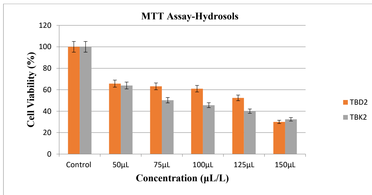
Figure 3. MTT Assay of Hydrosols of the Tapinanthus Species [TBD2= Tapinanthus bangwensis grown on Azadirachta indica ( IC_{50} =230.2357 \mu L/ml), TBK2= Tapinanthus bangwensis grown on Vitex doniana ( IC_{50} =46.4753 \mu L/ml)]
