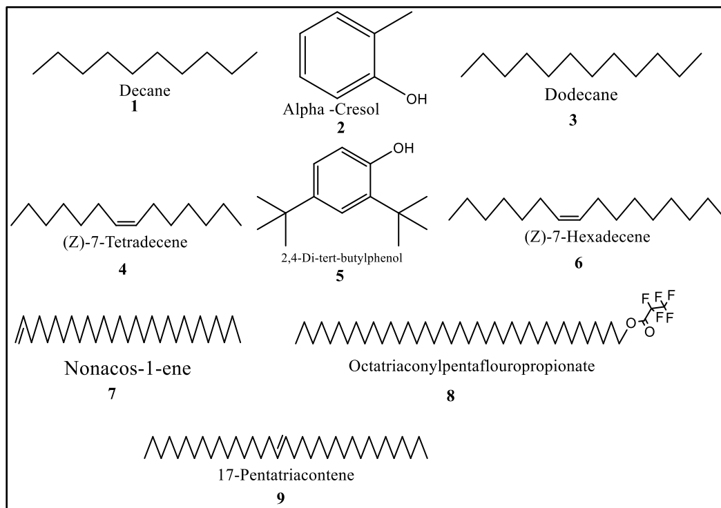
Figure 1. Structures of the Common Compounds in the Hydrosols
