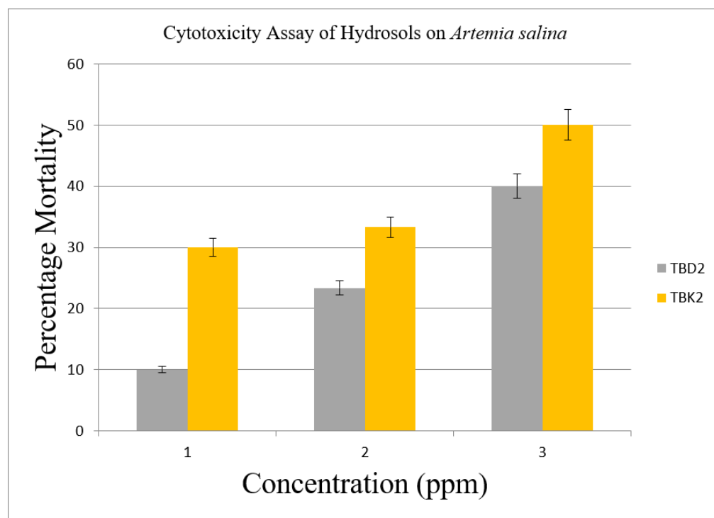
Figure 2. Cytotoxicity Assay of Hydrosols of the Tapinanthus Species [TBD2= Tapinanthus bangwensis grown on Azadirachta indica (LC 50 =2995.024 ppm), TBK2= Tapinanthus bangwensis grown on Vitex doniana (LC 50 =6672.169 ppm)]
